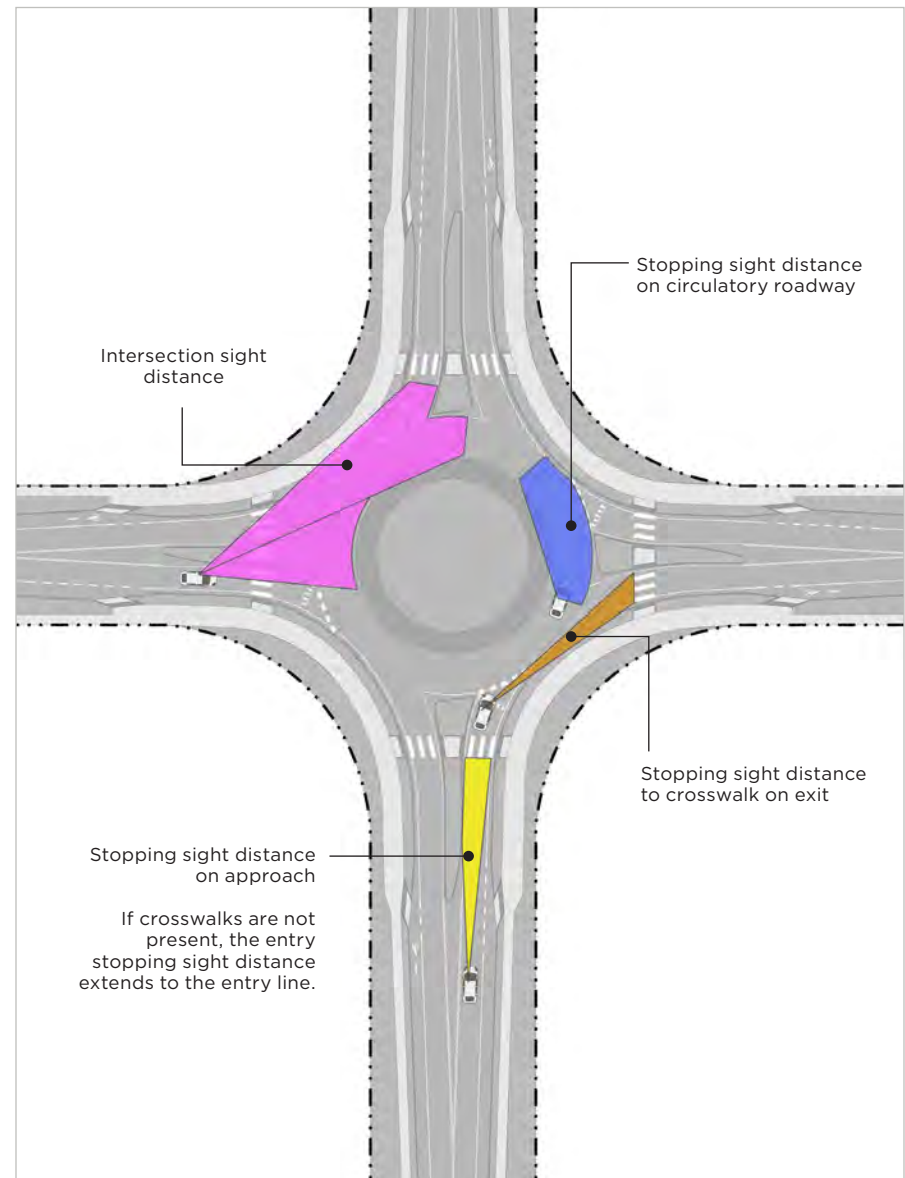
FIGURE 5-22: EXAMPLE SIGHT DISTANCE CHECKS
