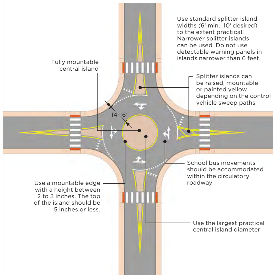
FIGURE 5-28: MINI-ROUNDBABOUT DESIGN ELEMENTS
