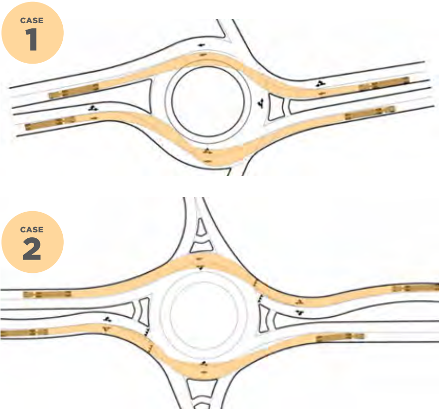
FIGURE 5-20: MULTILANE TRUCK ACCOMMODATION CASES
