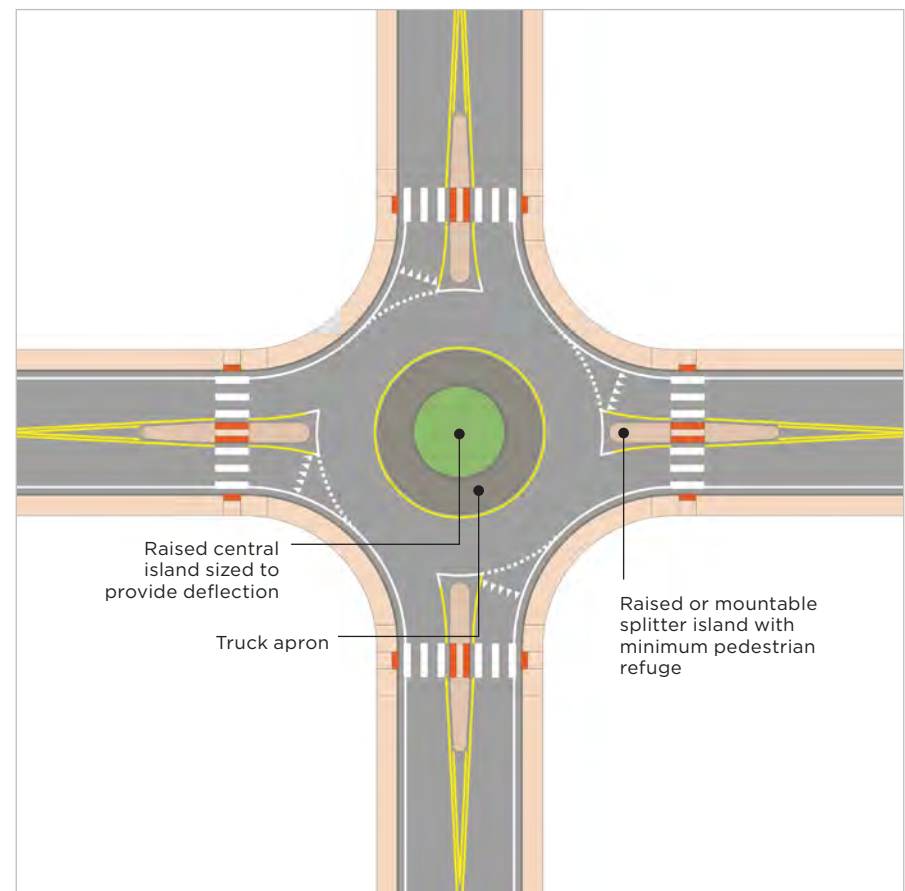
FIGURE 5-29: COMPACT ROUNDBABOUT DESIGN ELEMENTS
