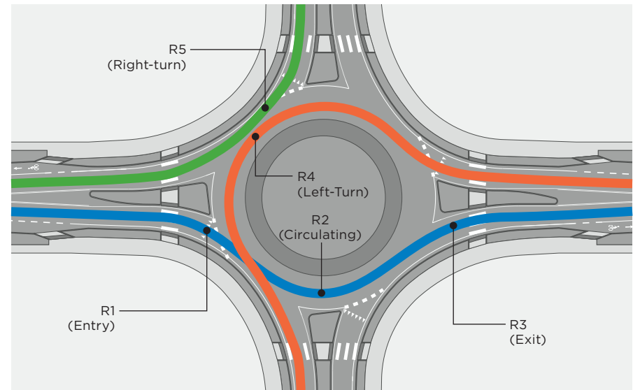
FIGURE 5-10: PERFORMANCE CHECKS RADII
