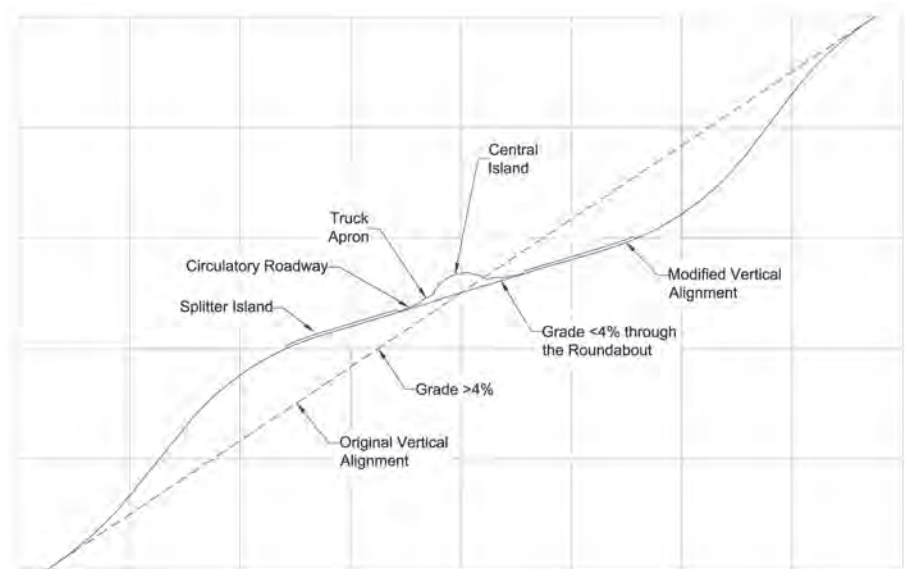
FIGURE 5-36: ROADWAY PROFILES AT A ROUNDABOUT
