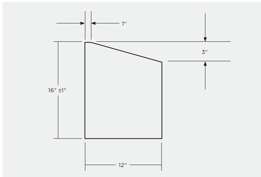
FIGURE 5-35: MOUNTABLE CURB DETAIL
