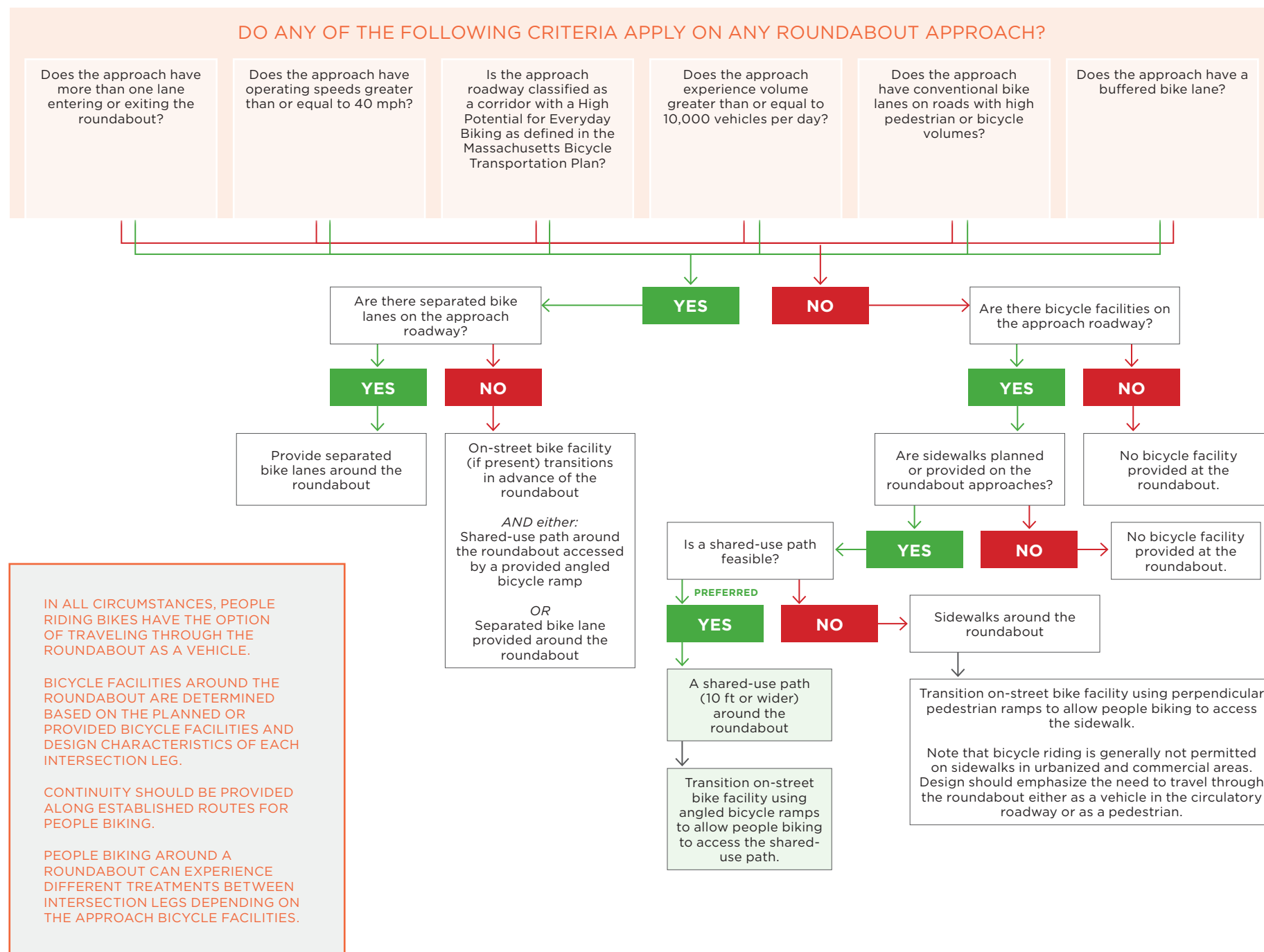
FIGURE 5-17: BICYCLE FACILITY OPTIONS AT A ROUNDABOUT
