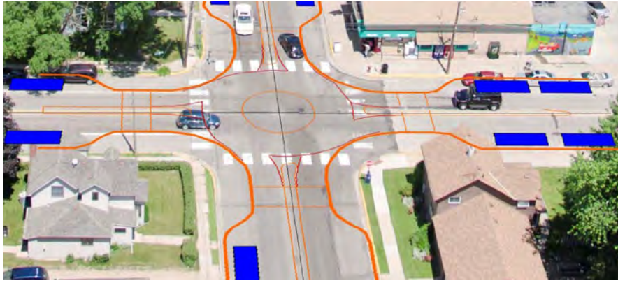
FIGURE 5-30: MINI-ROUNDBABOUT CURBS OUTLINE WITH AN EXISTING INTERSECTION AREA IN STILLWATER, MN
