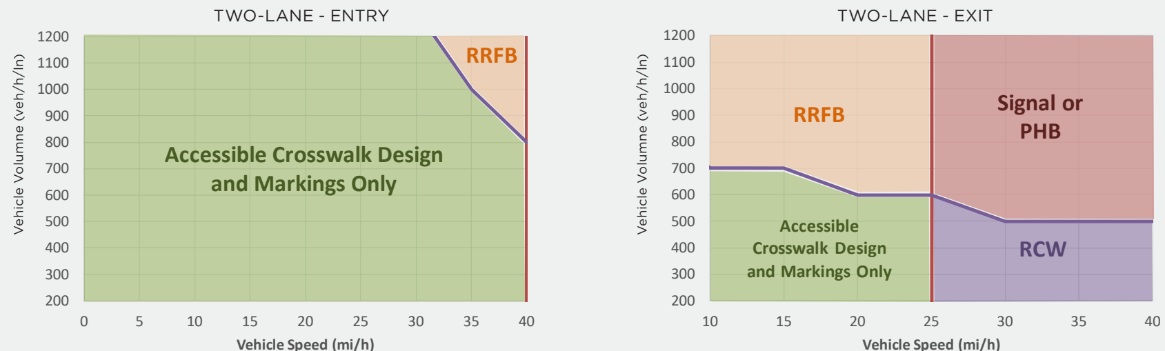
FIGURE 5-15: CROSSWALK TREATMENT RECOMMENDATIONS FOR TWO-LANE ROUNDABOUTS IN LOW NOISE ENVIRONMENTS
