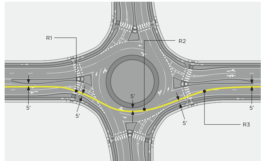
FIGURE 5-11: FASTEST VEHICLE PATHS THROUGH A MULTILANE ROUNDABOUT
