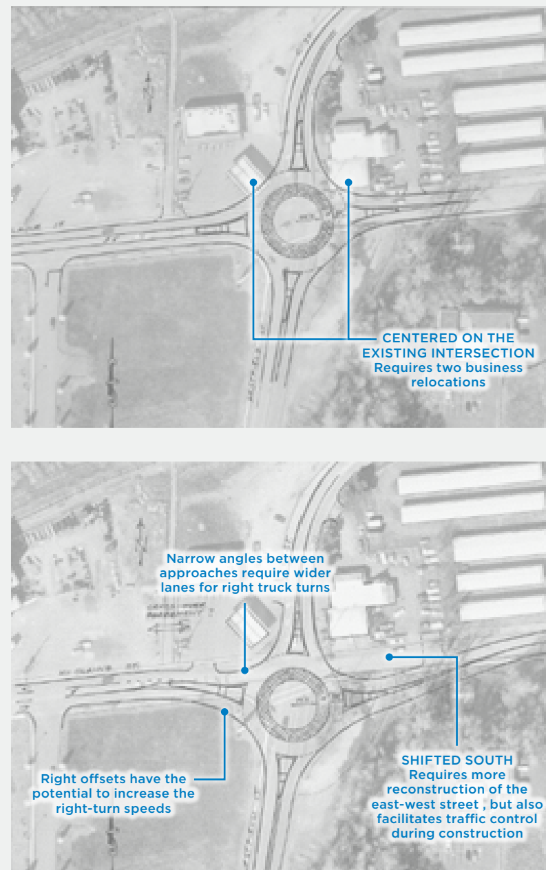
FIGURE 5-2: POTENTIAL OPTIONS FOR POSITIONING A ROUNDABOUT AT AN INTERSECTION
