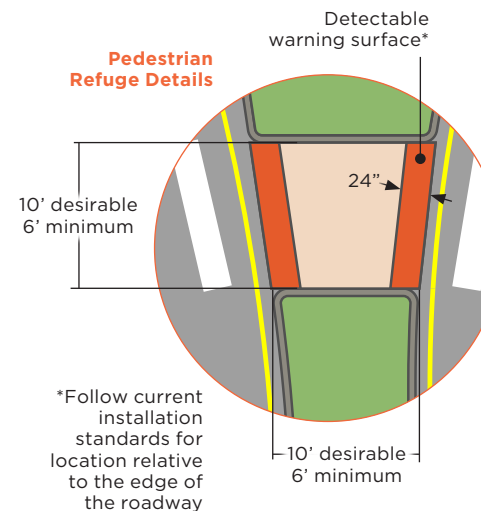
Mini-roundabout Splitter Island Details
