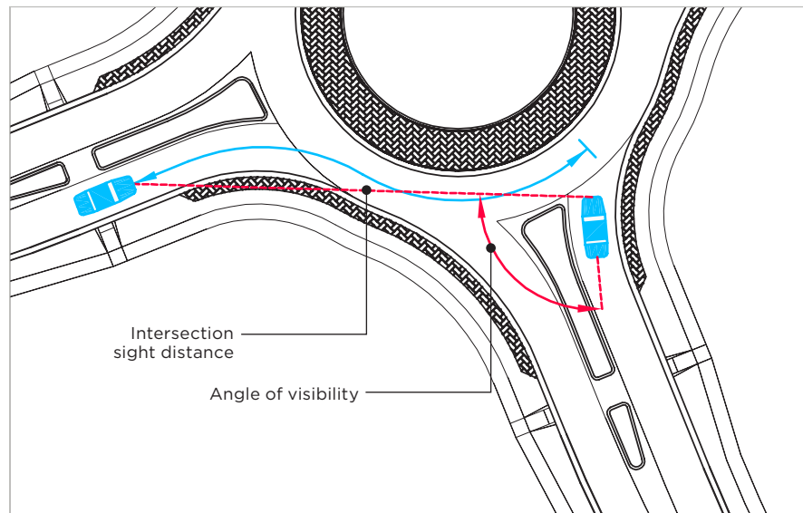
FIGURE 5-23: EXAMPLE ANGLE OF VISIBILITY CHECK
