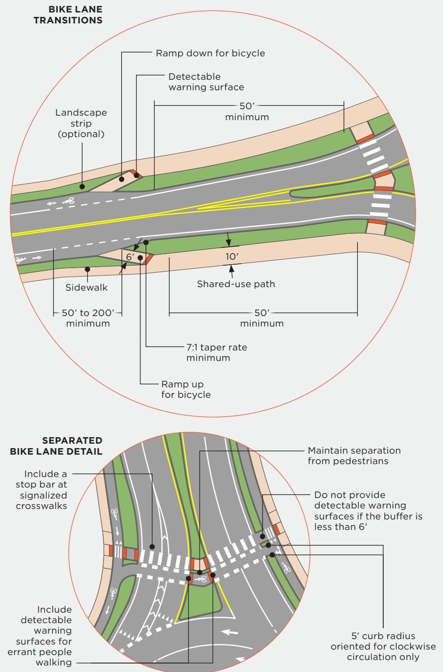
FIGURE 5-16: PEDESTRIAN AND BICYCLE FACILITIES DETAILS
