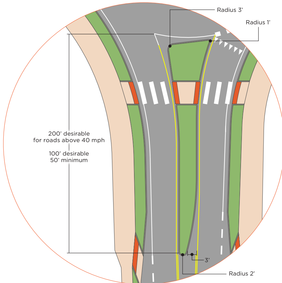
FIGURE 5-9: SPLITTER ISLAND ELEMENTS AND DIMENSIONS
