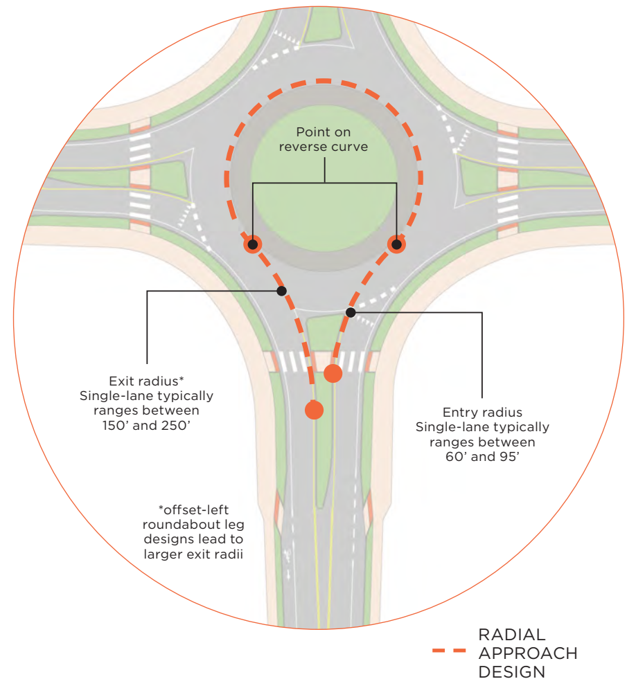
FIGURE 5-5: SINGLE-LANE ROUNDABOUT LEG GEOMETRY ELEMENTS
